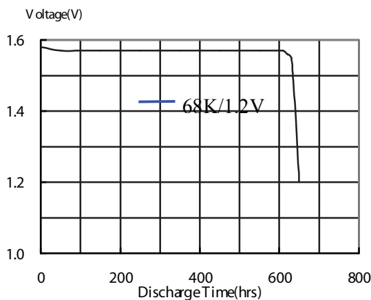
Typical Discharge characteristics at 20 ± 2°C
