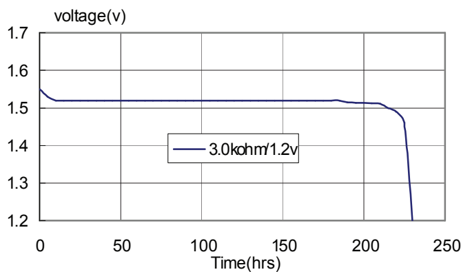
Typical Discharge curve at 20±2°C
