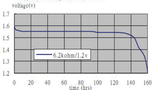
Typical discharge curve at 20±2°C
