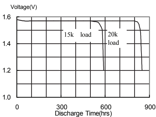
Typical Discharge characteristics at 20 ± 2 °C
