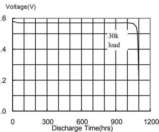
Typical Discharge characteristics at 20 ± 2 °C
